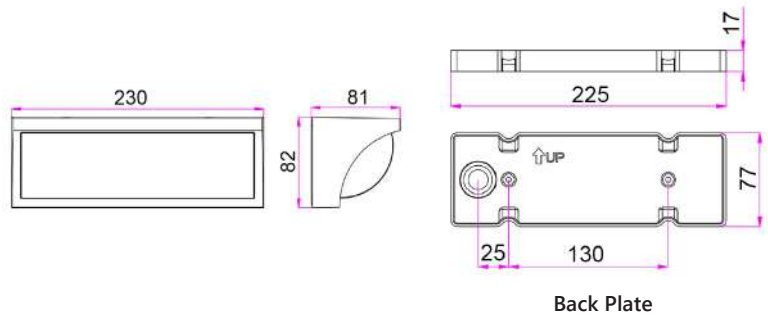
Back Plate
