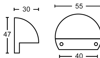
STE10 (Brass Nickel Plated)
