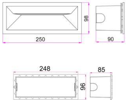
Sleeve line drawing
