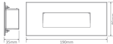
Cutout: 160mm x 68mm
