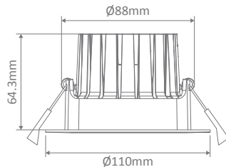
Cutout: Ø90-95mm
