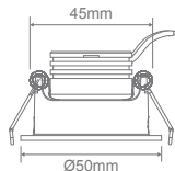
Cutout: Ø45mm - Tilt: 20° Driver fits through cutout hole
