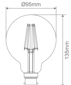
LF-G95-FRS-B22
