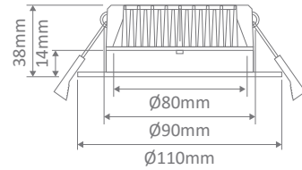
Cutout: Ø90mm
