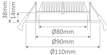
Cutout: Ø90mm
