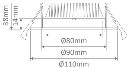
Cutout: Ø90mm
