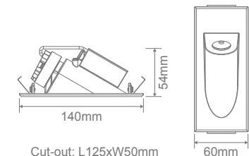
Cut-out: L125xW50mm
