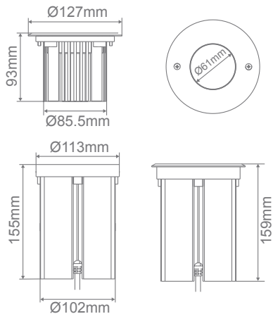
Cutout: Ø110-120mm
