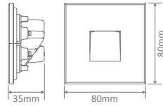
Cutout: \phi 68mm
