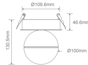
Cutout: Ø110mm
