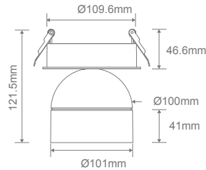
Cutout: Ø110mm
