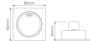
Depth without recessed box: (D) 46mm Cutout without recessed box: (Ø) 70mm
