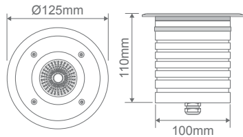
Cutout: Ø110mm
