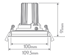
Cutout: L100mm x W100mm
