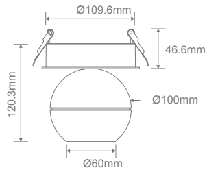
Cutout: Ø110mm
