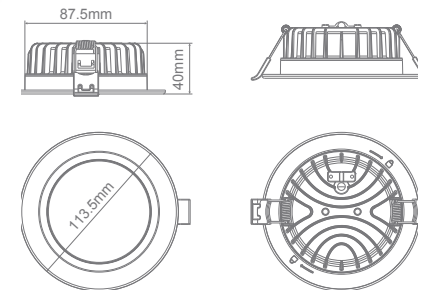
Cutout: 90mm
