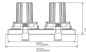
Cutout: L190mm x W100mm
