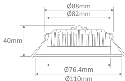
Cutout: Ø90mm
