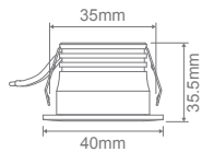
Cutout: Ø35mm Driver fits through cutout hole
