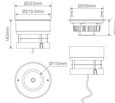
Cutout: Ø205-215mm
