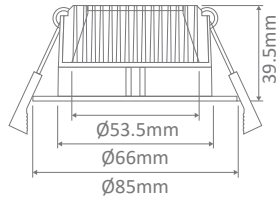
Cutout: Ø70-75mm
