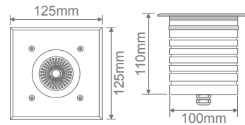
Cutout: Ø110mm
