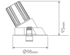
Cutout: \varnothing 88-90\text{mm} W90 wall washer frame is set at a 45° angle.
