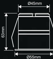
Cutout: Ø50mm Driver fits through cutout hole
