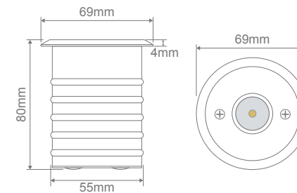
Cutout: Ø60-65mm
