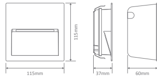
Cutout without recessed box: (Ø) 100mm Cutout with recessed box: (L) 110mm x (H) 110mm
