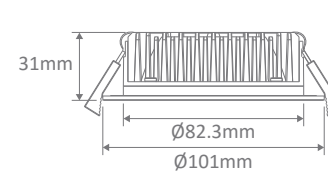
Ø90mm Cutout
