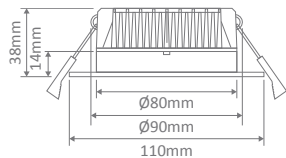
Cutout: Ø90mm
