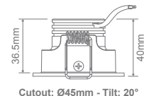
Cutout: Ø45mm - Tilt: 20° Driver fits through cutout hole
