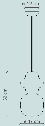
art. C2681 peso netto / net weight 2,12 1 x MAX 28W E14
