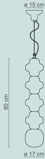
art. C2682 - C2685 peso netto / net weight Kg 5,00 1 x MAX 28W E14
