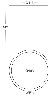
HV5803T-BLK-EXT HV5803T-BLK-EXT-12V
