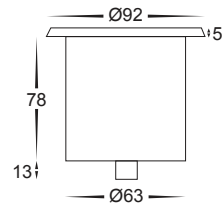
Cutout without Canister Ø63
