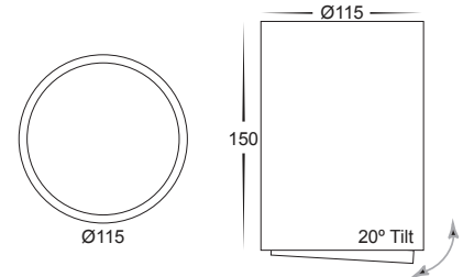
HV5815T-WHT HV5815T-WHT-12V
