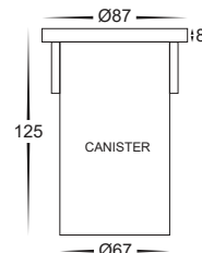
Cutout with Canister Ø87
