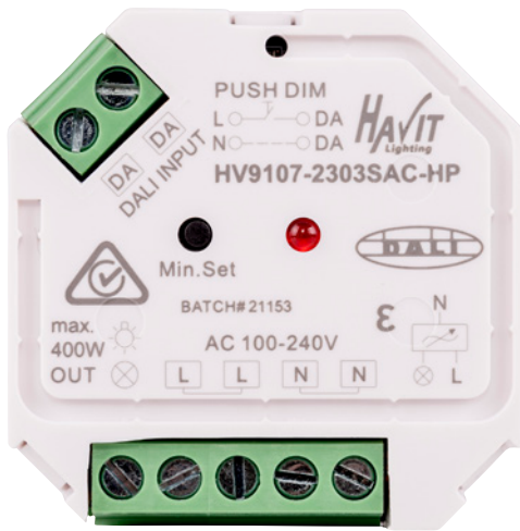
Dimming Relay HV9107-2303SAC-HP
