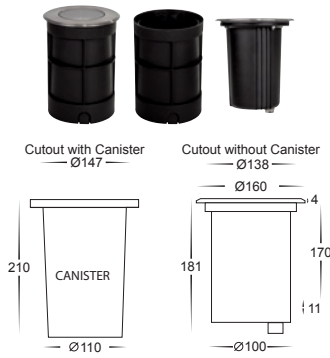
Face: 160mm Tilt: 30° HV1828T
