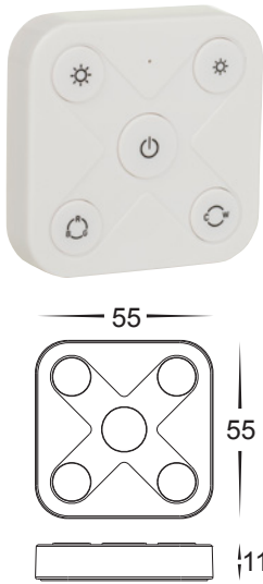
Zigbee Wireless Wall Switch HV9101-ZB-5C
