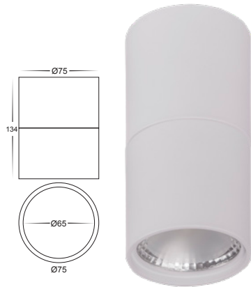
HV5802T-WHT-EXT HV5802T-WHT-EXT-12V
