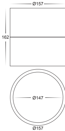
HV5805T-BLK-EXT HV5805T-BLK-EXT-12V
