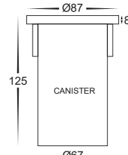
Cutout with Canister Ø87
