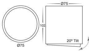
HV5812T-WHT HV5812T-WHT-12V
