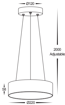
HV5892T-BLK-PDT HV5892T-WHT-PDT
