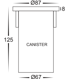
Cutout with Canister Ø87
