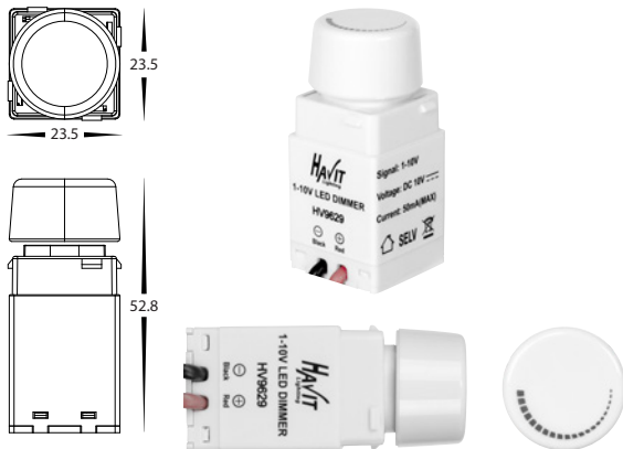
1-10v LED Strip Dimming Pot HV9629
