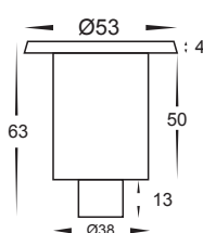
Cutout without Canister — Ø38 —
