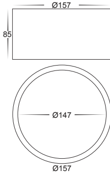
HV5805T-BLK HV5805T-BLK-12V
