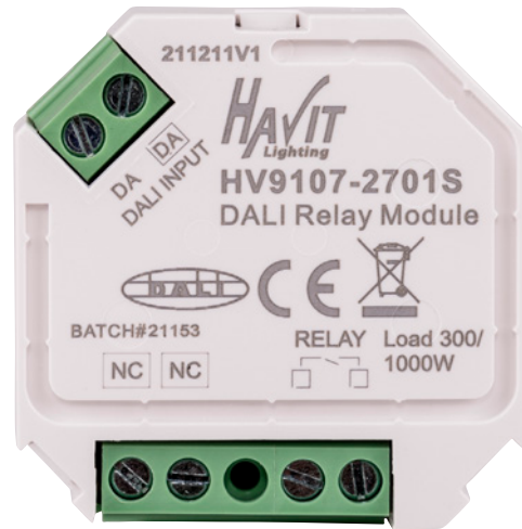
On/Off Relay HV9107-2701S
