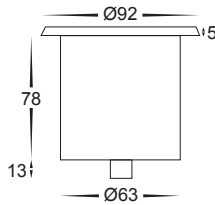
Cutout without Canister Ø63
